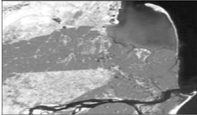
Fig. 3.6 Supervised classification :
