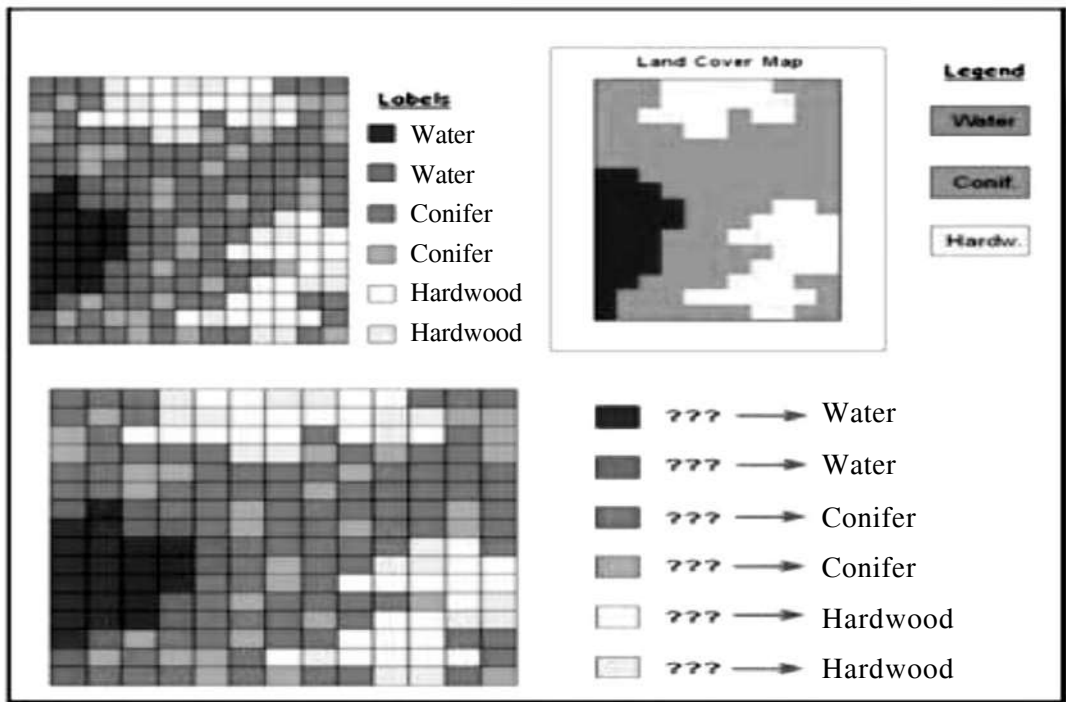
Fig. 3.5 Unsupervised classification :
